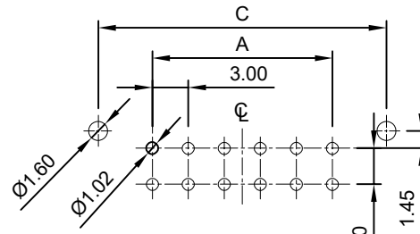
P.C.B LAYOUT: TOP VIEW TOLERANCE: ±0.05mm
