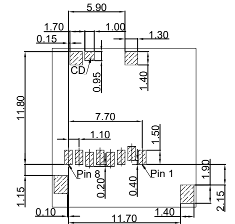
RECOMMENDED PCB HOLE LAYOUT COMPONENT SIDE VIEW (TOLERANCE: ±0.05)
